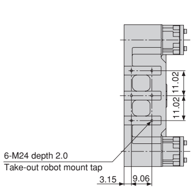
Upper surface of stationary platen
