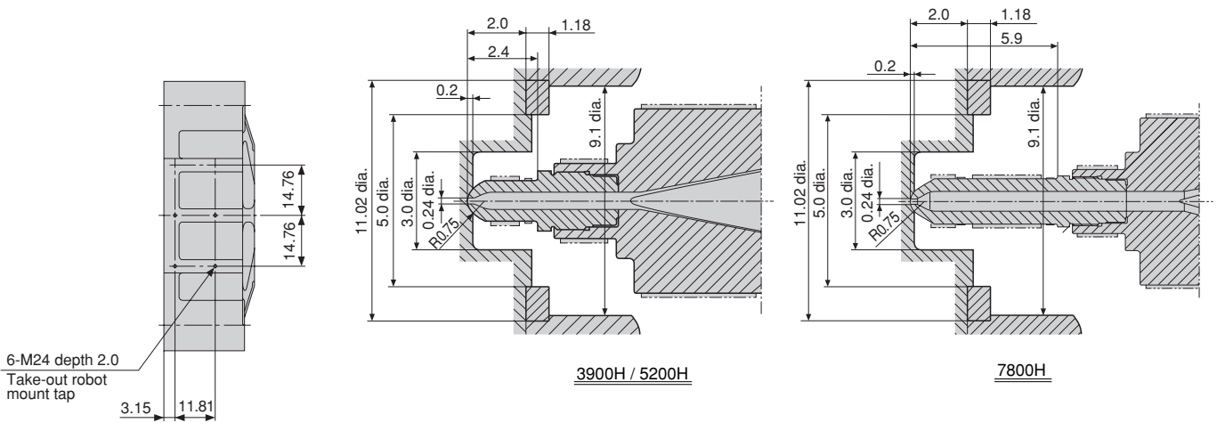
Upper surface of stationary platen
